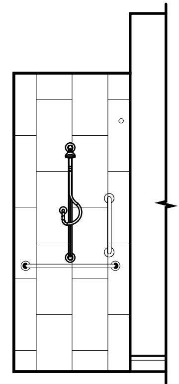
7 - BATHROOM ELEVATION
