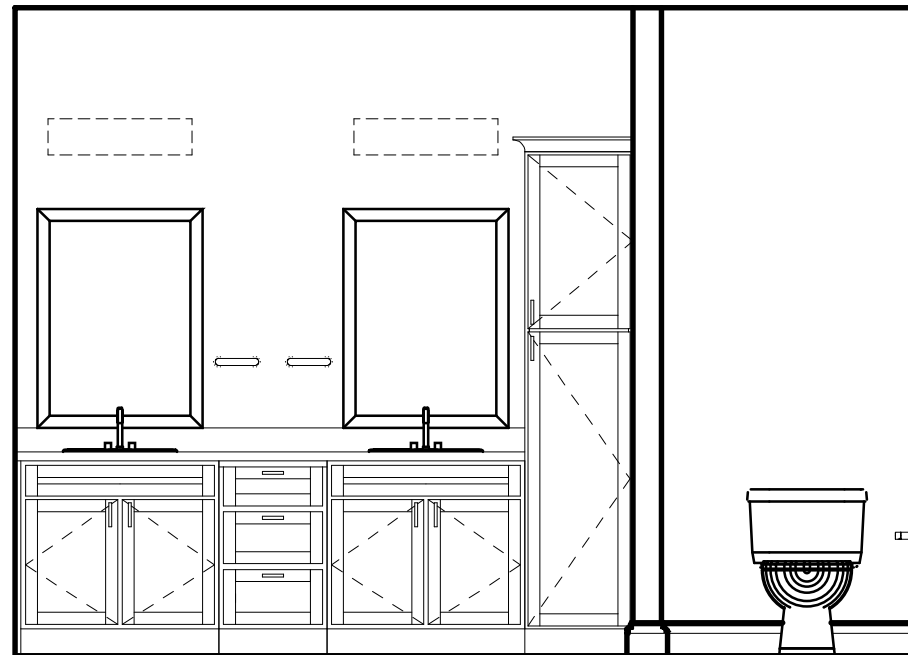
8 - BATHROOM ELEVATION
