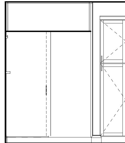
11 - BATHROOM ELEVATION
