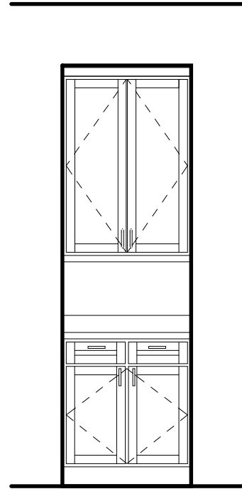
1 - KITCHEN ELEVATION
