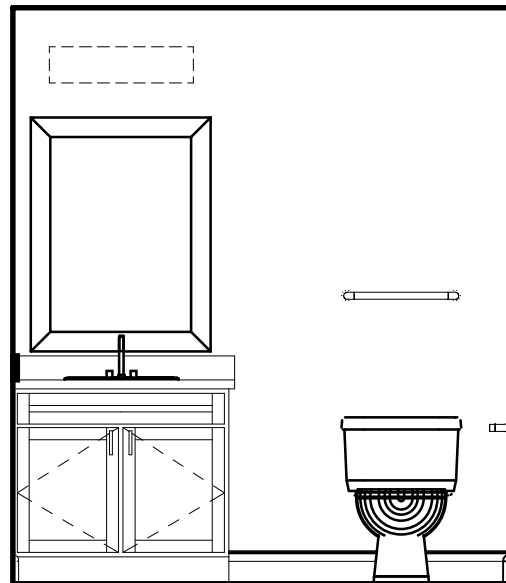
10 - BATHROOM ELEVATION
