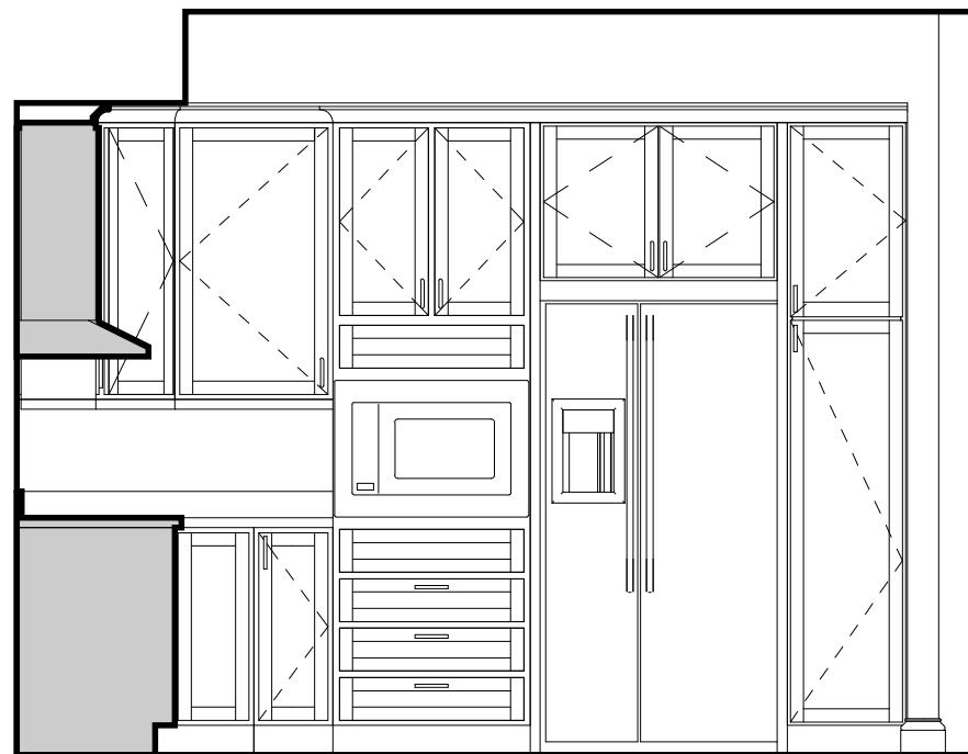
4 - KITCHEN ELEVATION
