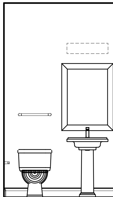
5 - BATHROOM ELEVATION
