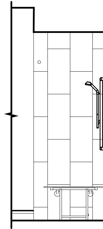
7 - BATHROOM ELEVATION
