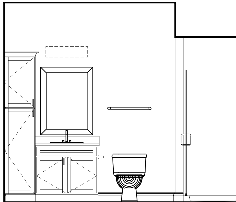
5 - BATHROOM ELEVATION
